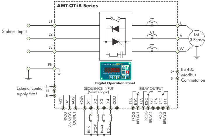
In-line configuration
